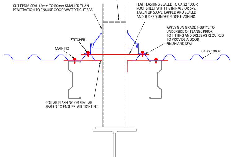
ROOF STUB STEELWORK PENETRATION DETAIL
